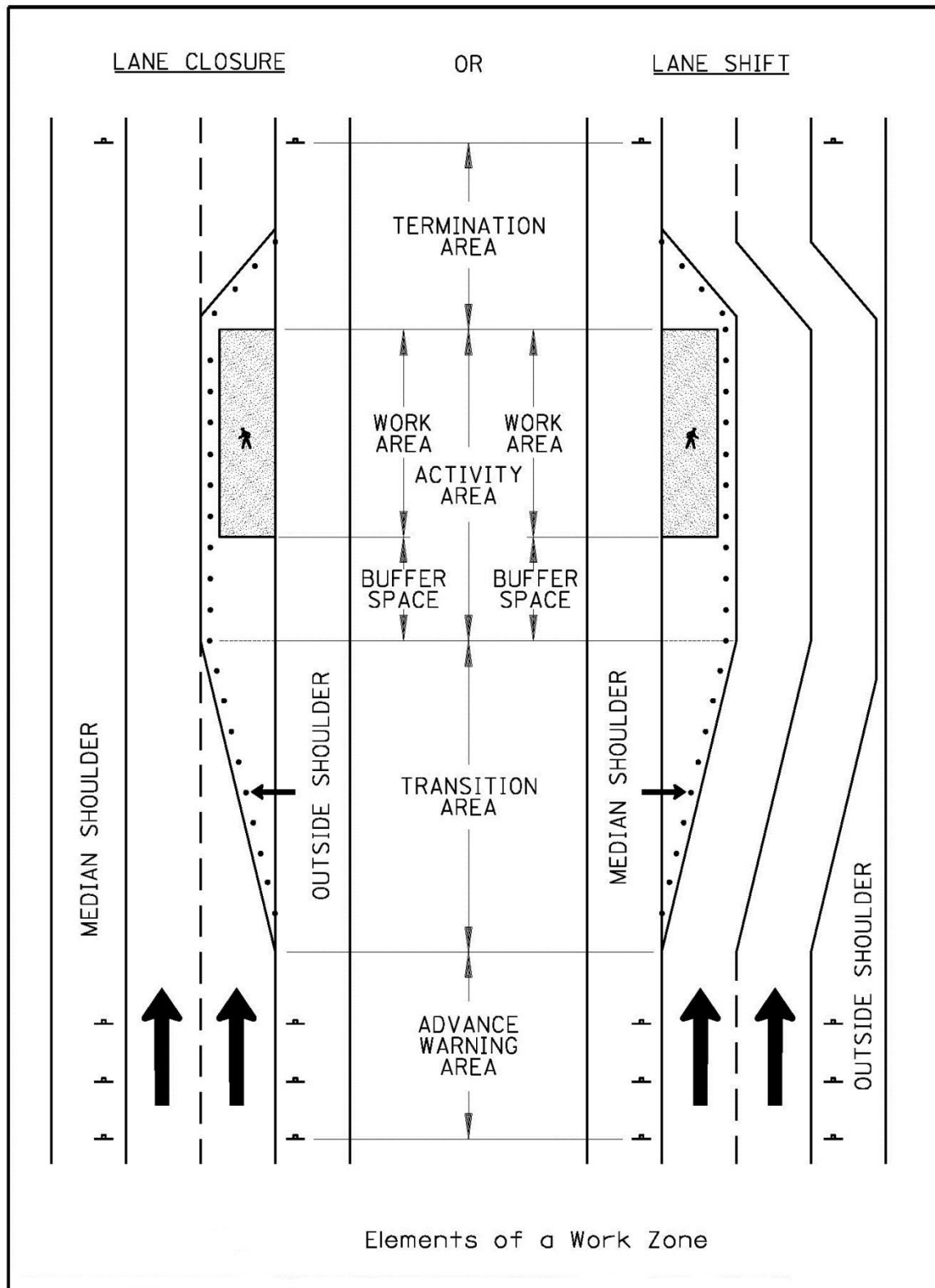
Figure 2 – Element of a Work Zone
