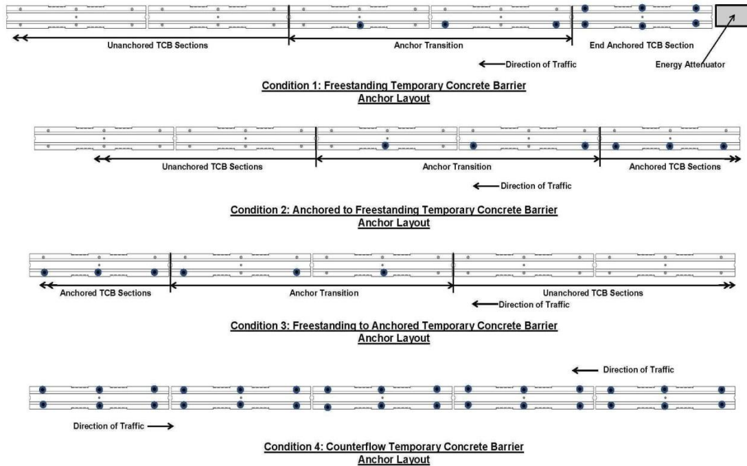
Figure 3 – Temporary Concrete Barrier Layouts
