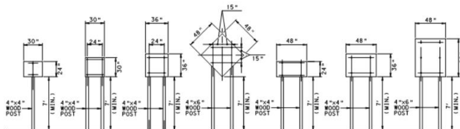
Figure 16. Typical wood sign post sizes for common sign types (PennDOT Pub 111, 2013)
