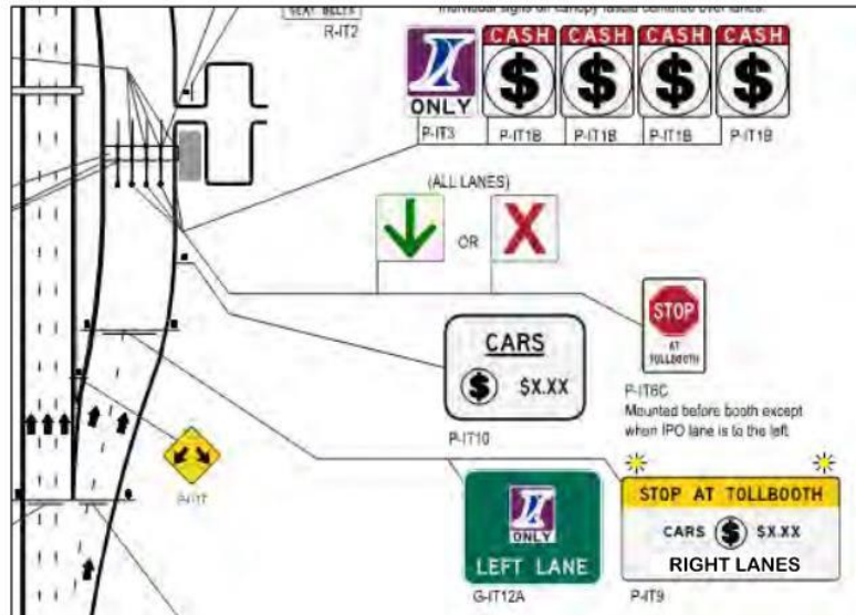
Figure 2 – Illinois Tollway Manual Side Signing Guidelines
