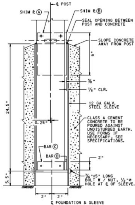
Figure 15. Example galvanized steel sleeve and concrete footing detail for wood posts (PennDOT Pub 111, 2013)
