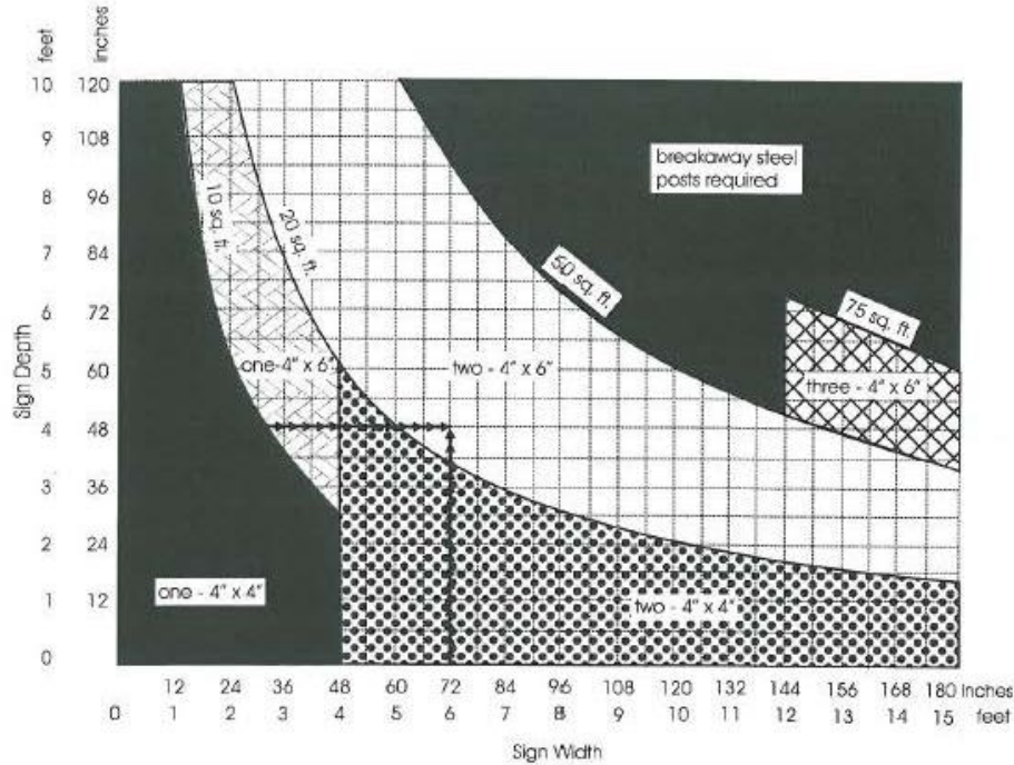
Determination of sign post size and number
