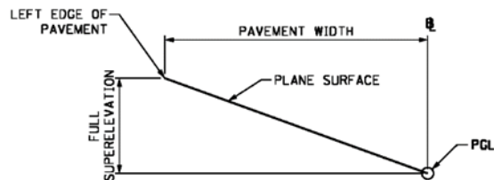
SECTION G-G
