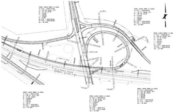
Figure 4.3 L300-L350 visual
