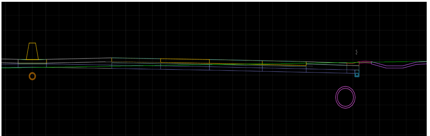
L200 roadway pavement, L200 MSE wall, L300 grading, L300 underground utilities
