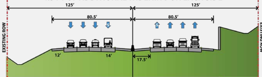
SHORT TERM - ADD LANE AS MANAGED LANE 4.5 FT OF ADDITIONAL WIDENING ON EACH SIDE
