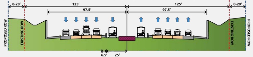
LONG TERM - AT FUTURE STATION LOCATIONS
