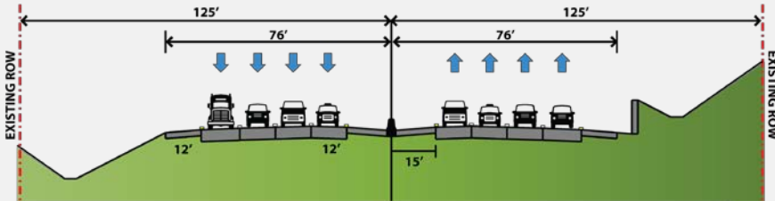
SHORT TERM - ADD LANE AS MANAGED LANE 4.5 FT OF ADDITIONAL WIDENING ON EACH SIDE
