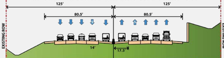
MID-TERM - ADDITIONAL TRANSIT COMPONENT - BOS
