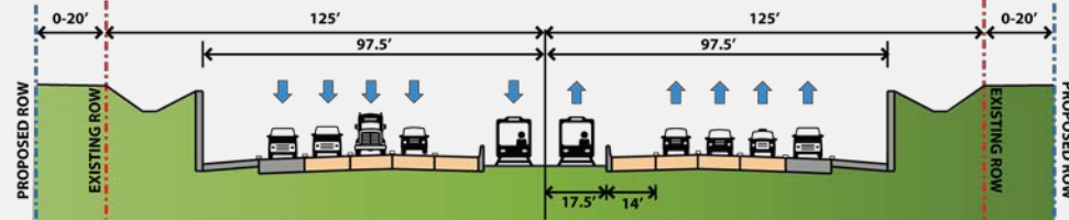
LONG TERM - BETWEEN STATIONS
